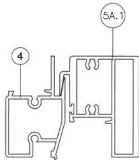
HEAVY DUTY TOP RAIL S-1000
